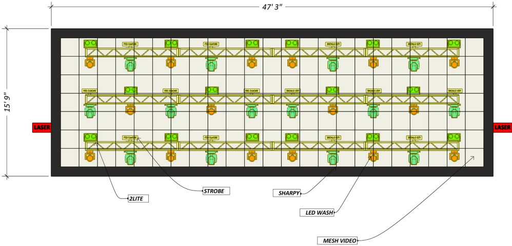
DDA-01 Upstage Center Display - Front View scale: 1/4" = 1'
